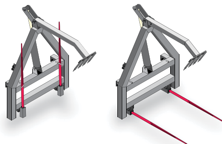
Folding hay bale spike with top spike
