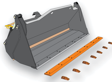
4 in 1 cereals bucket
