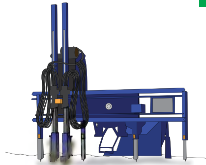
Block paving compaction system
