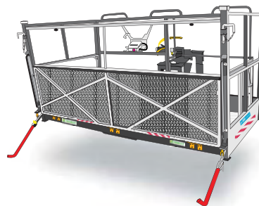
Front-opening slewing platform
