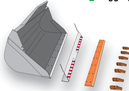
Digging bucket
