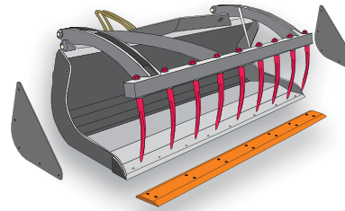
General purpose bucket and grab
