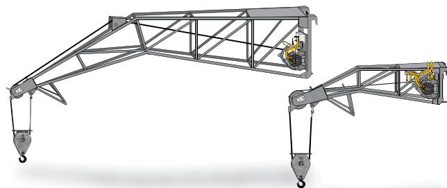
Lattice jib with winch
